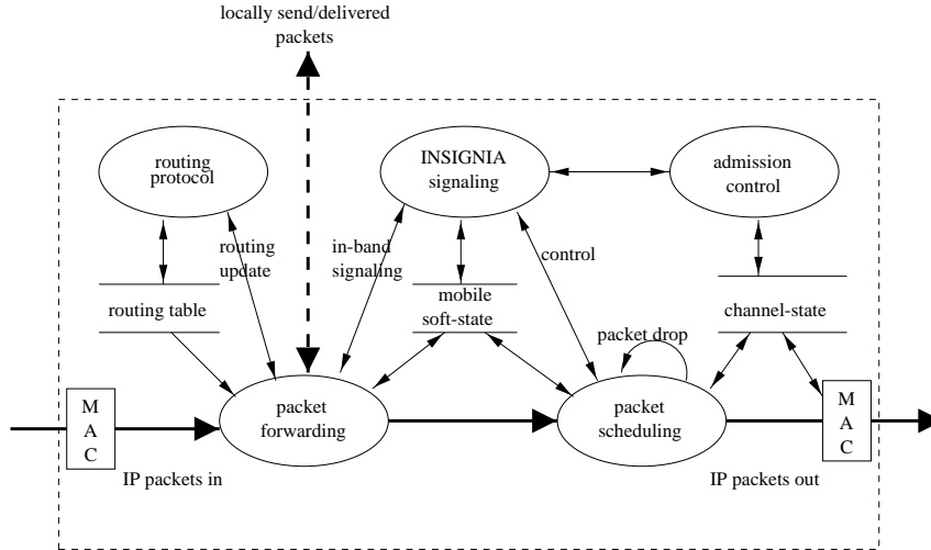
Figure 4: The INSIGNIA framework.
