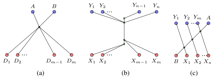
Fig. 3: Combinations of X-Sets
