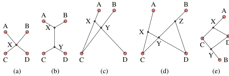
Fig. 2: Different Combinations of Two "Y"s.
